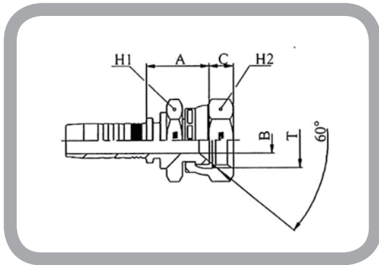
M23811- JIS BSP Female 60° Cone Seat (Toyota) - JIS B 8363 (Crimped Back Nut)
