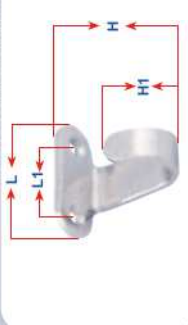
Art. n° 8372 Gancio multiuso Coat hook, polished
